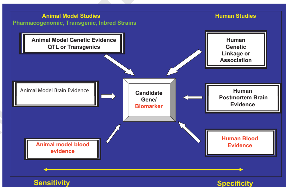
Figure 1. Convergent functional genomics: multiple independent lines of evidence for Bayesian integration.
